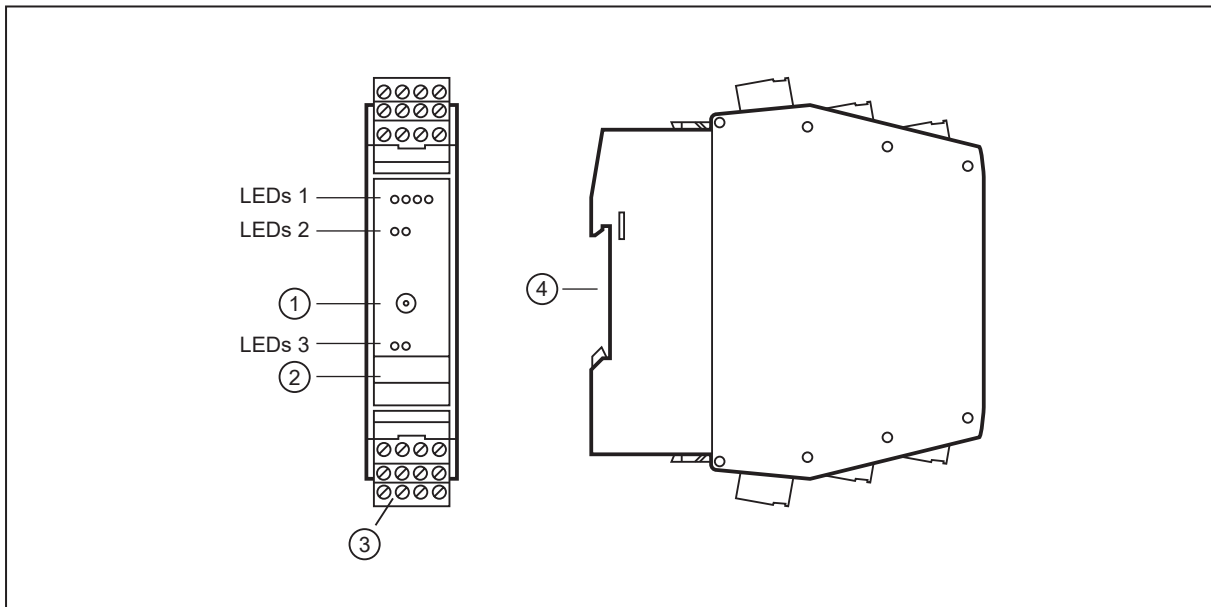
Fig. 7: LED assignment AC2256
