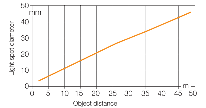
Fig. 5: Light spot diameter depending on distance to the object
